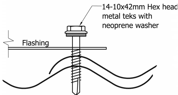
Figure 3 – Fixing Details.
