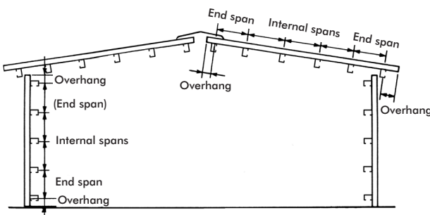
Figure 2.14.A End Spans, Internal Spans and Overhangs
